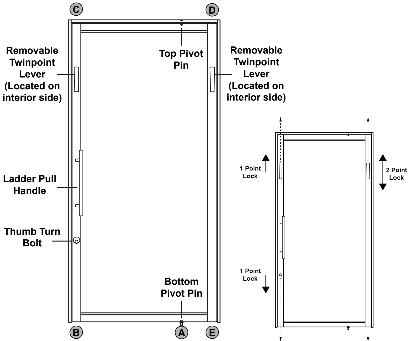
(EXTERIOR VIEW)
